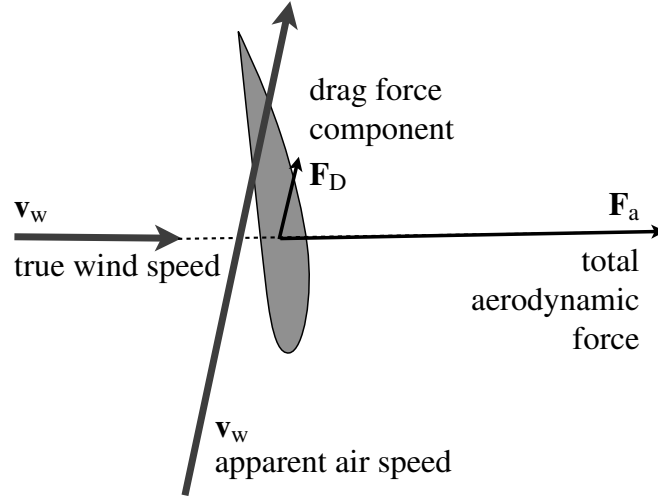
Fig. 1.6 Sketch of the relevant speeds and forces around a wing for wind power generation.
