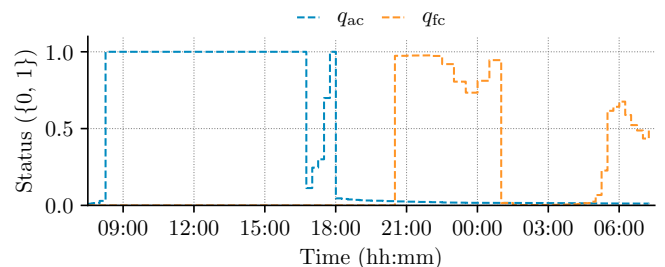
Fig. 3. Depiction of the relaxed solution.
